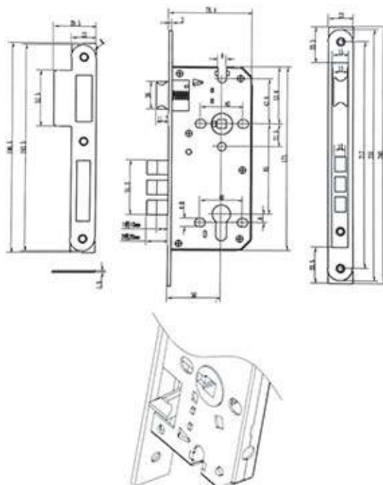
Reversing Diagram
