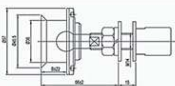
ETG-T01 Articulated Routel - Normal (57mm)
