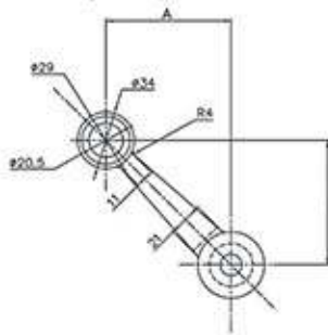
ETG204-1-90 One Way Clamp
