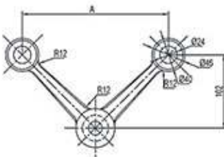
ETG204-2-90 Two Way (90) Clamp
