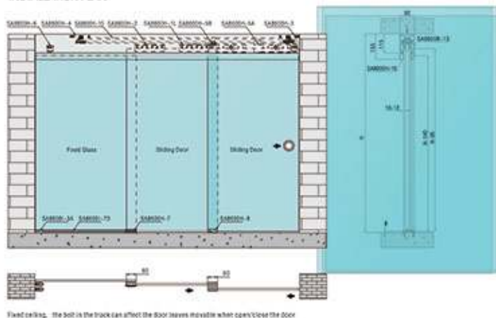
INSTALLATION PLAN
