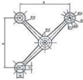
ETG204-3 Three Way Clamp
