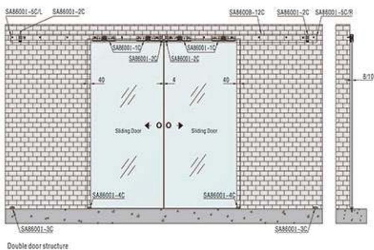
INSTALLATION PLAN
