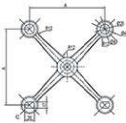
ETG204-4 Four Way Clamp
