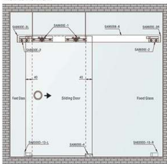
Single door structure
