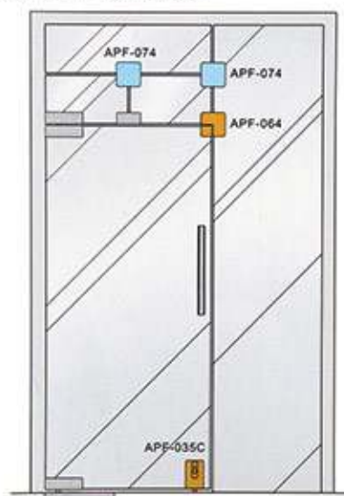
EAPF-074 Top Patch for connecting 4 glass panels
