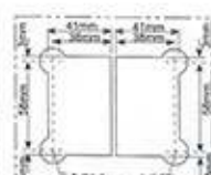
Glass to Glass Hinge 90
