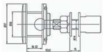
ETG-T03 Articulated Routel - Counter Sunk
