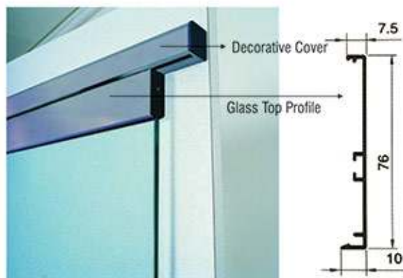
Glass Top Profile
