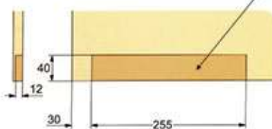
Roller Cutout Dimensions
