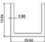
Bottom Track Cross Section :
