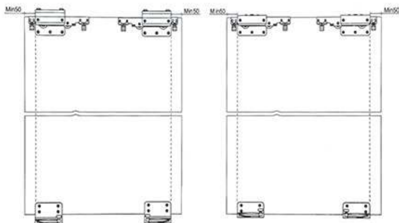
Door Back View (Roller Positions)
