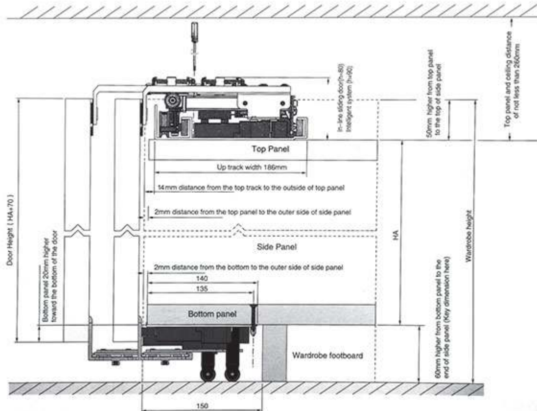
Installation Details: Carcass Side View
