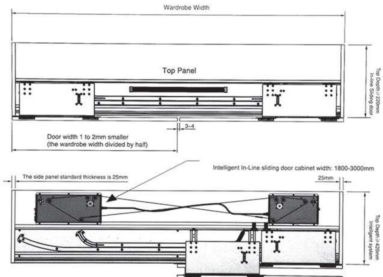
Installation Details: Carcass Top View
