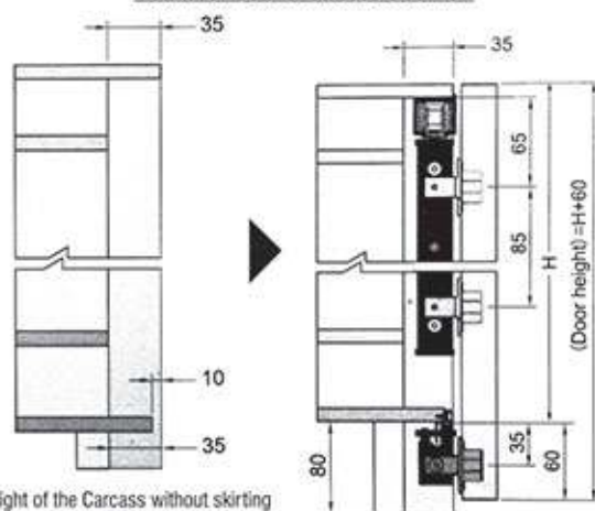
Installation Details: Carcass Side View
